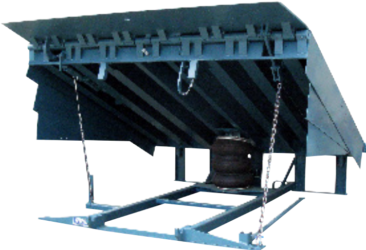
CentraAir® Series, 6' x 8', 45,000 CIR, Shown patent pending
